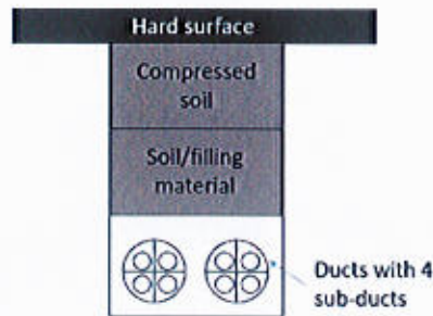
Figure 2: Generic representation of Omantel's trench with sub-ducts
